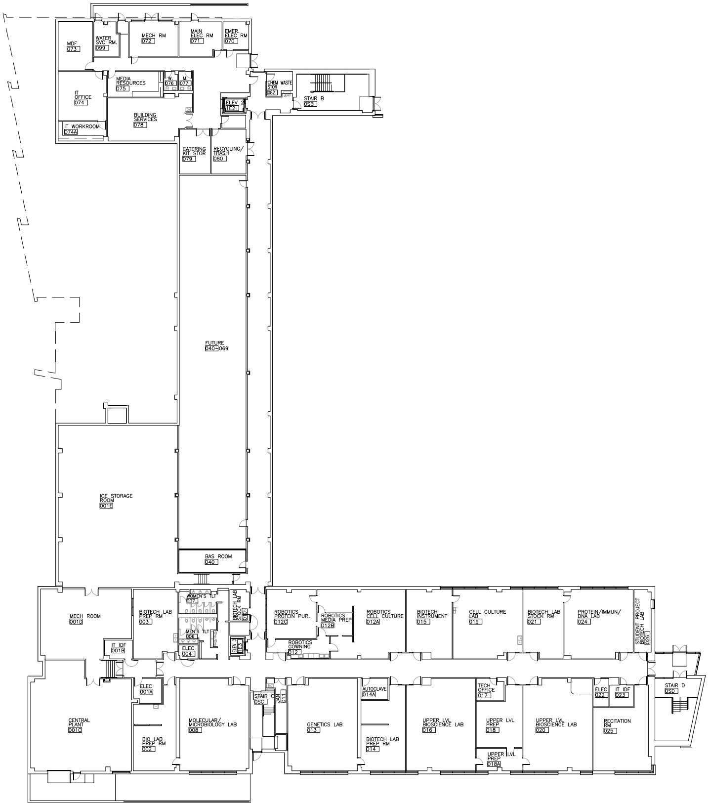
LOWER LEVEL PLAN
